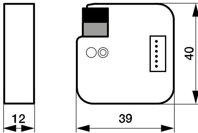
Fig. 1: Dimension drawing
